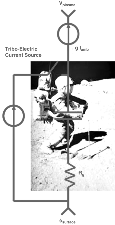
Fig. 1 Astronaut charging equivalent circuit model (Farrell et al. [11]).
